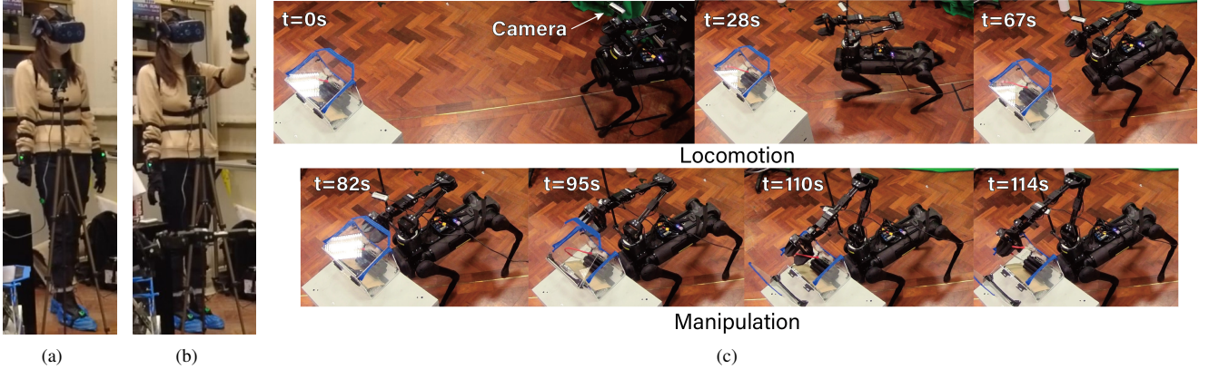
Fig. 2: The operator uses (a) lower body for locomotion and (b) upper body for manipulation control of (c) a legged manipulator in an EOD experiment.
